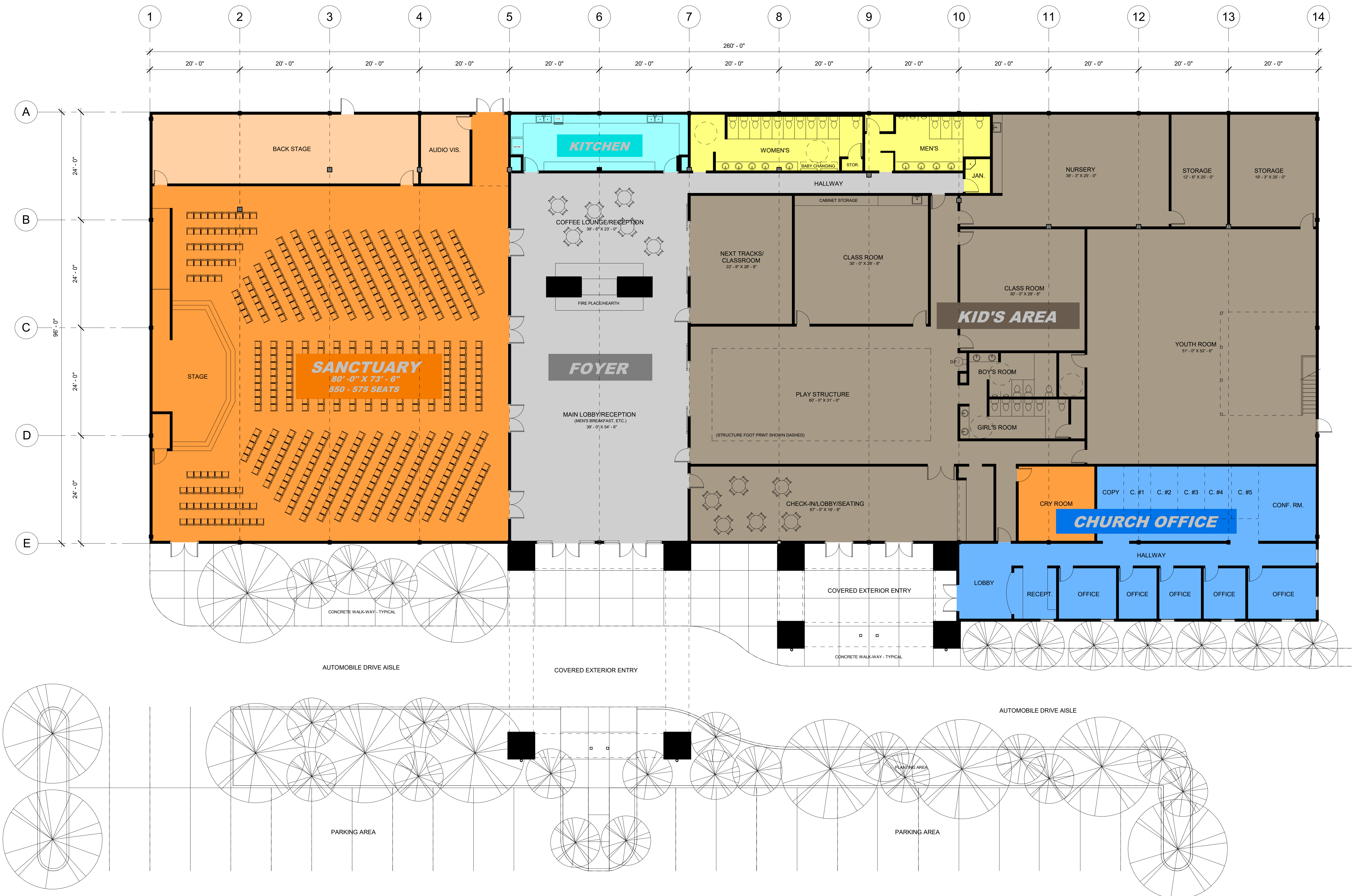
JOY CHURCH SCHEMATIC FLOOR PLAN APRIL 04.2019 1" = 10'-0" 1
